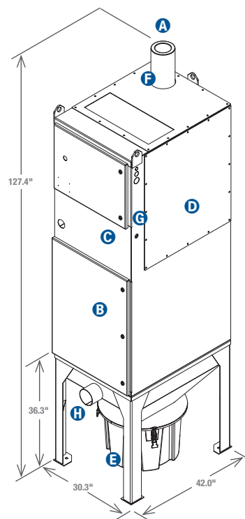
HDH Hopper
