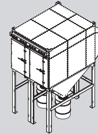
RDC-4X5-20C CFM Range: 4670-42030 Unit Weight: 7613 SCFM: 20
