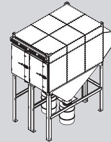
RDC-4X6-24C CFM Range: 5604-50436 Unit Weight: 10018 SCFM: 20
