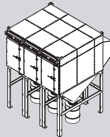
RDC-6X5-30C CFM Range: 7005-63045 Unit Weight: 11144 SCFM: 23
