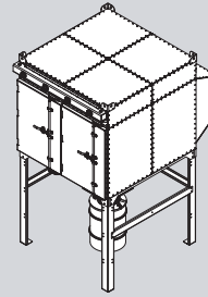
RDC-4X4-16C CFM Range: 3736-33624 Unit Weight: 6546 SCFM: 20
