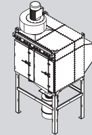
RDC-4X3-12C CFM Range: 2802-25218 Unit Weight: 3908 SCFM: 20
